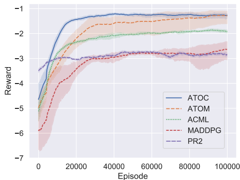
Figure 3: Learning Curve of Cooperative Navigation.
