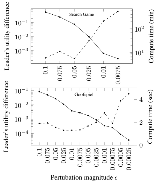
Figure 3: Experiments. Dashed lines shows compute time. Solid lines shows the loss in the leader’s utility compared to the SSE value in the unperturbed game.
